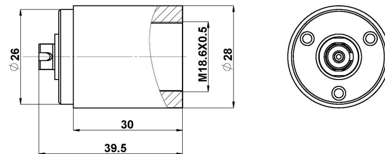
FC Connector
