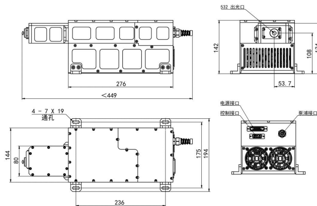
449 (L)×144 (W)×142(H) mm 3 , 5kg
